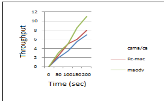
Figure:3 The graph representing throughput comparison
